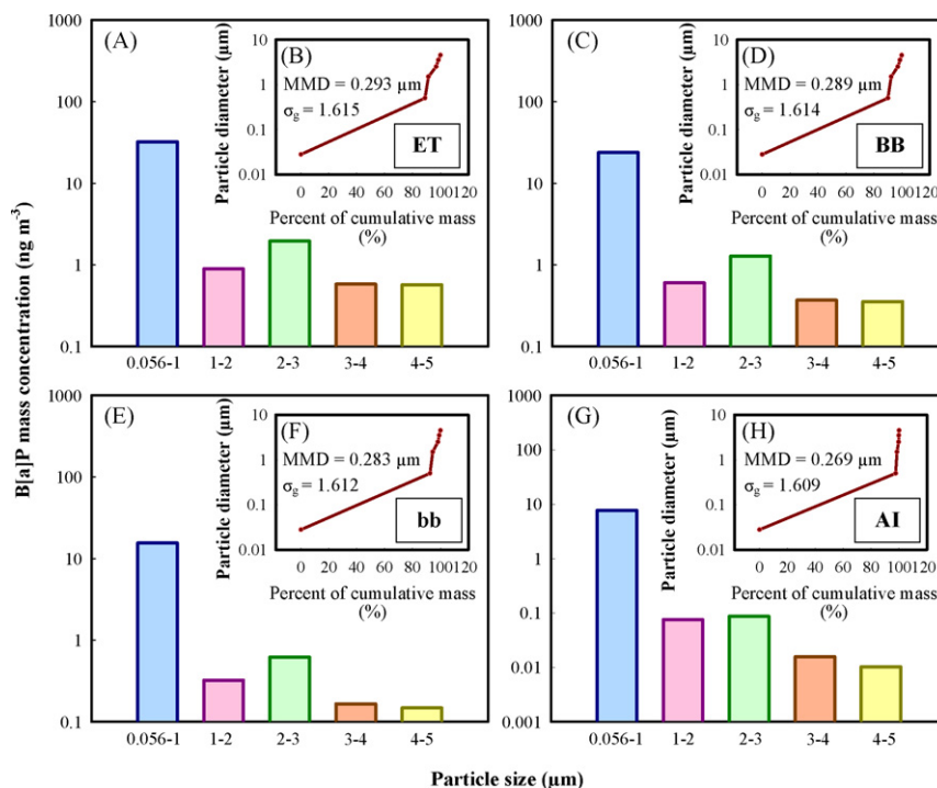
Fig. 2. Steady-state concentration distribution and size distribution patterns of B[a]P in different HRT regions: (A, B) ET, (C, D) BB, (E, F) bb, and (G, H) AI.
